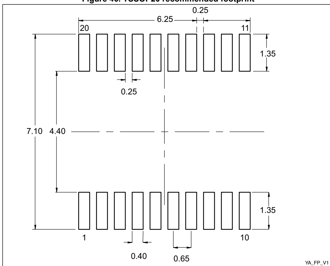
Figure 46. TSSOP20 recommended footprint
