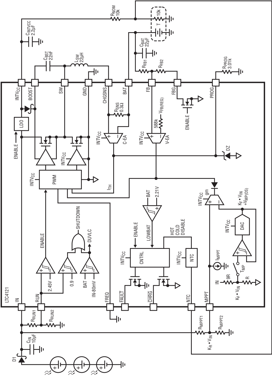
Figure 1. Block Diagram
