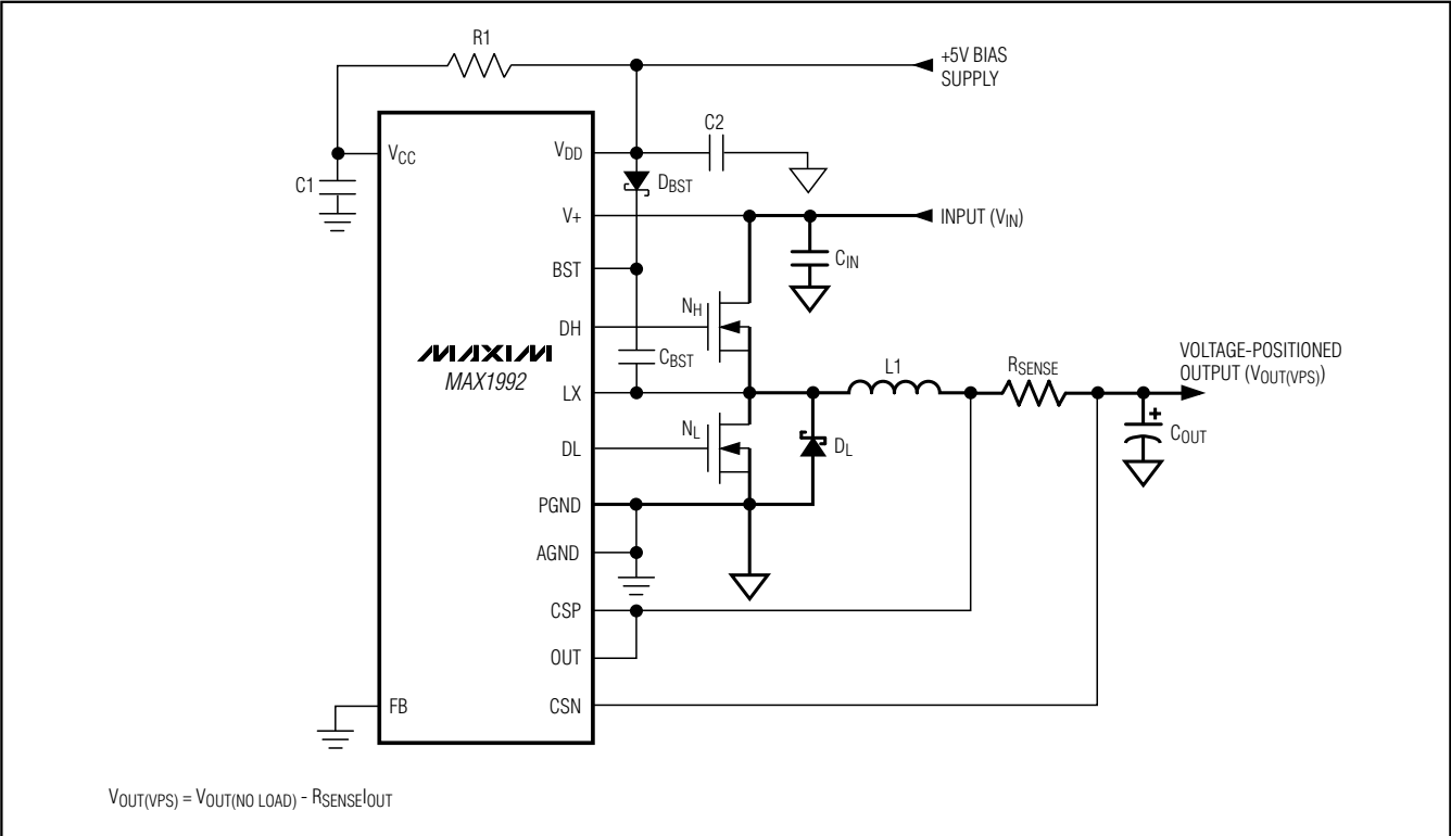
Figure 13. Voltage-Positioning Output
