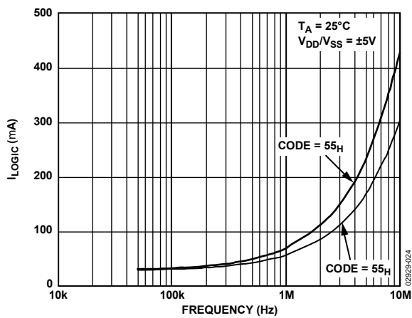
Figure 26. V_{\text{LOGIC}} Supply Current vs. Frequency
