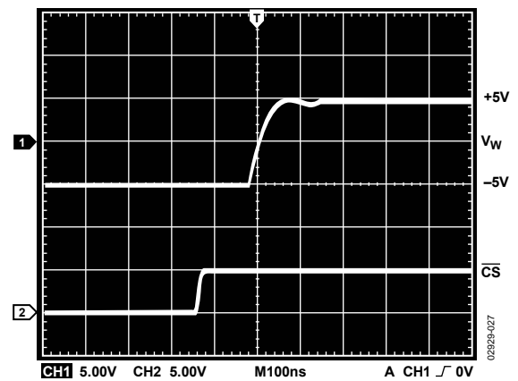
Figure 29. Large Signal Settling Time
