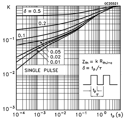
Derating Curve
