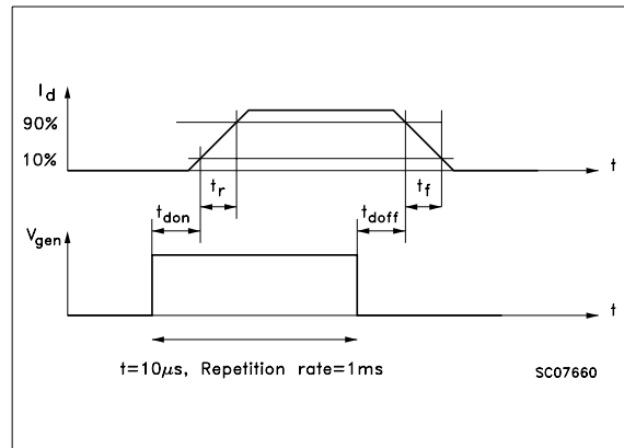
Figure 6: Waveforms
