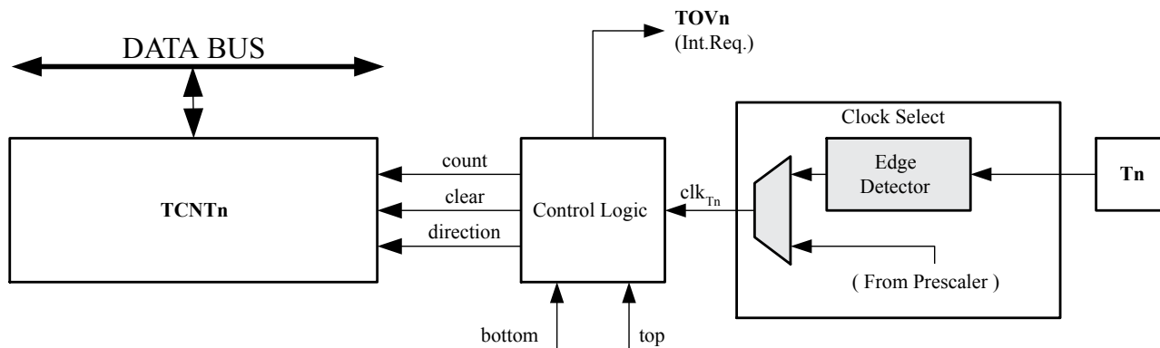
Figure 15-2. Counter Unit Block Diagram
