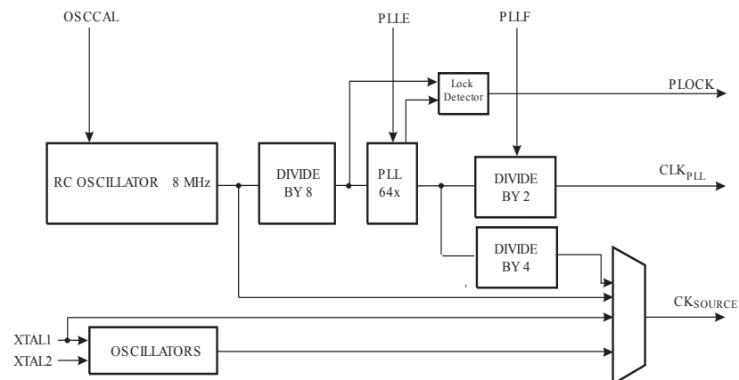
Figure 9-3. PCK clocking system
