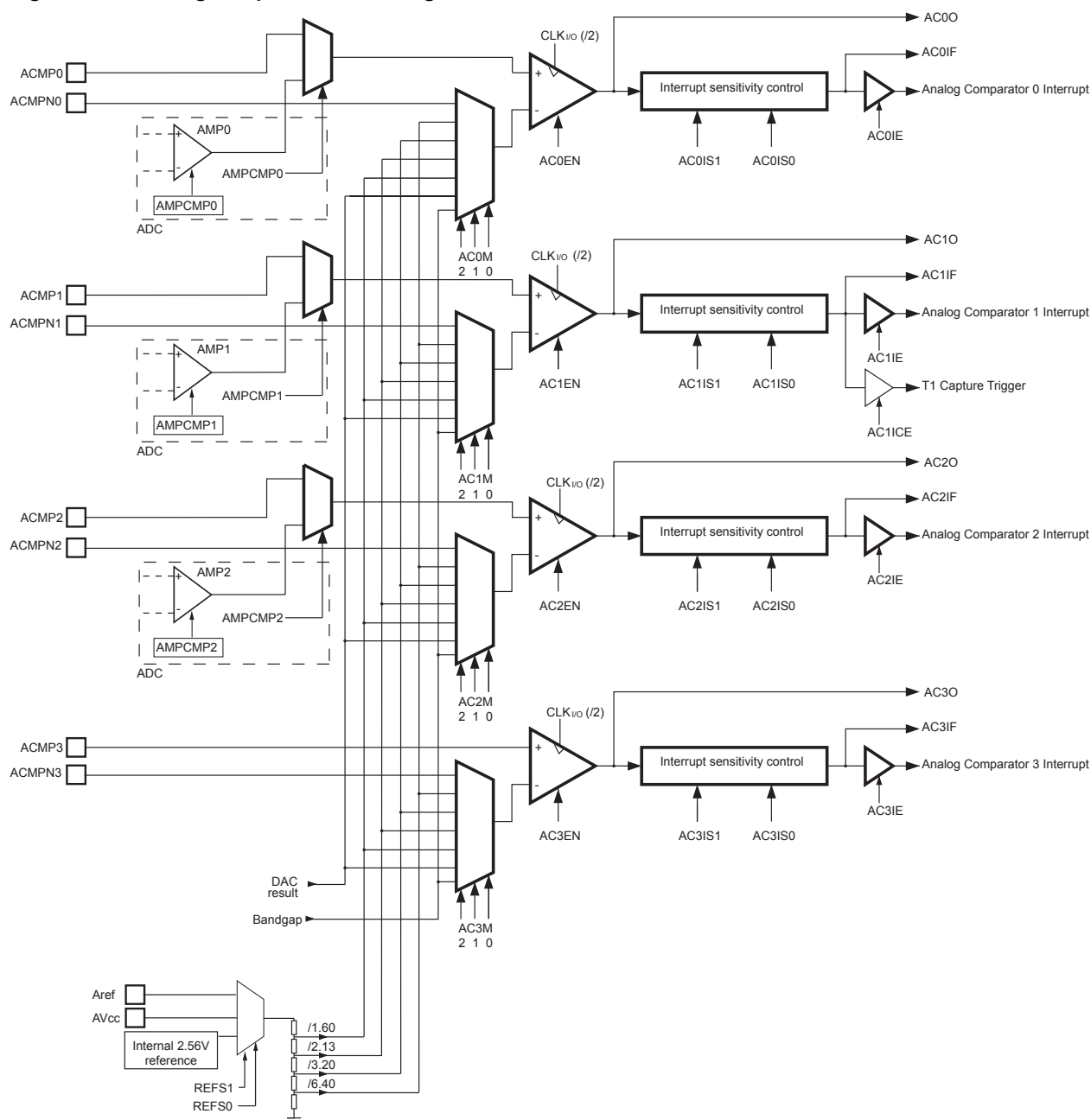
Figure 24-1. Analog comparator block diagram
