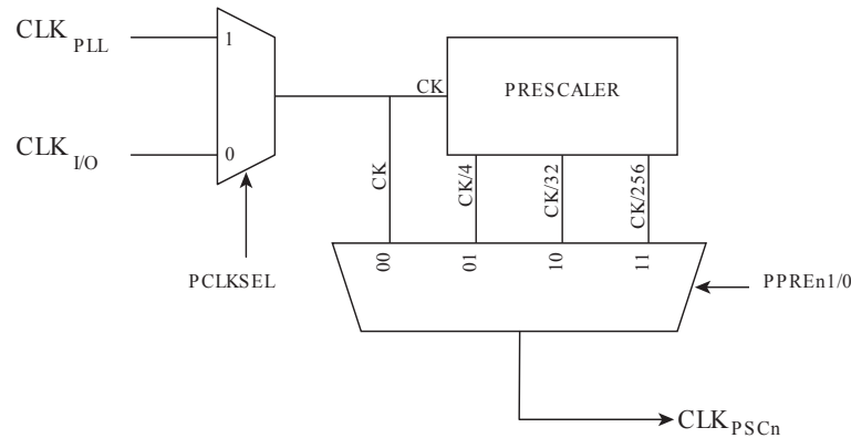
Figure 18-15. Clock selection.
