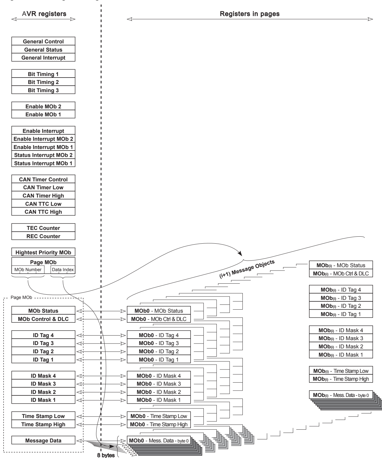
Figure 20-15. Registers organization
