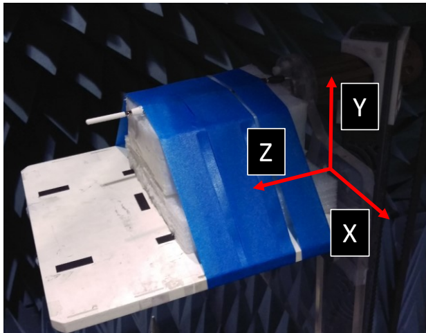
Chamber Setup
