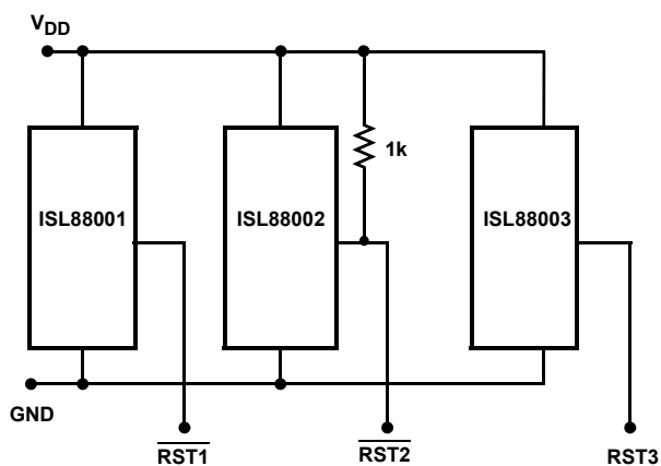
FIGURE 13. ISL88001/2/3EVAL1Z SCHEMATIC
