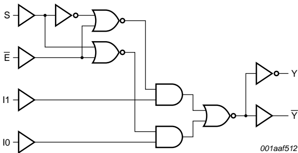
Fig 4. Functional diagram
