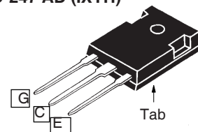
TO-247 AD (IXYH)
