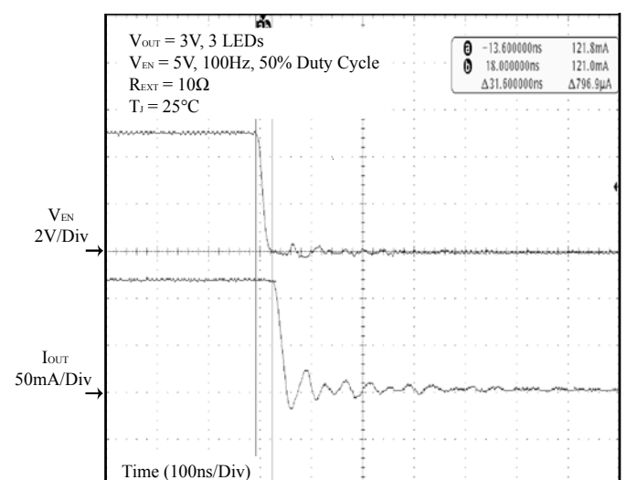
Figure 32 V_{EN} vs. I_{OUT} Delay and Falling Edge
