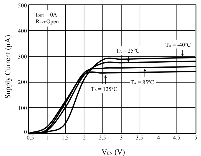
Figure 26 I_{EN} vs. V_{EN}
