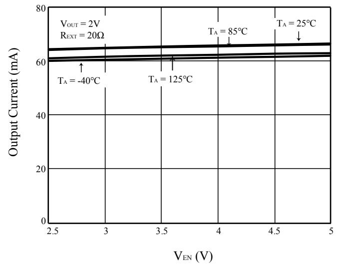
Figure 22 I_{OUT} vs. V_{EN}
