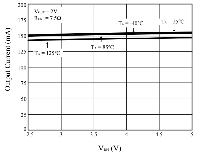
Figure 24 I_{OUT} vs. V_{EN}
