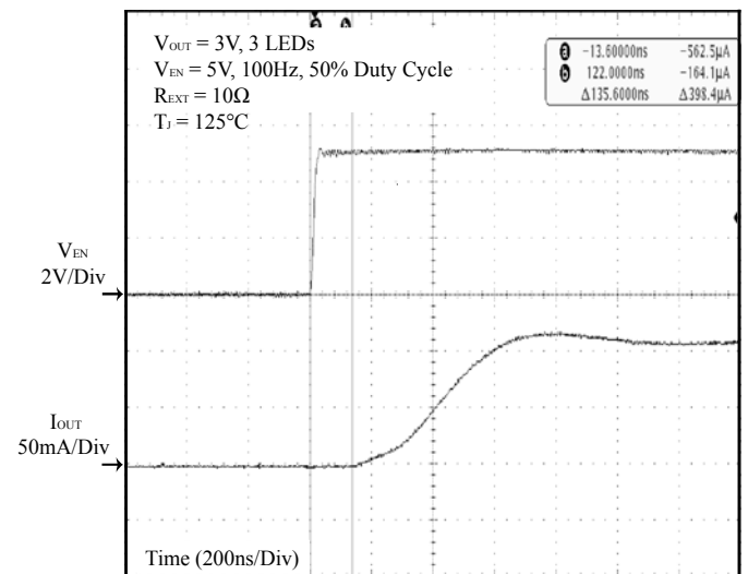
Figure 30 V_{EN} vs. I_{OUT} Delay and Rising Edge
