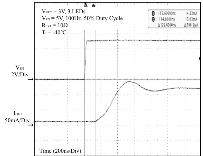
Figure 28 V_{EN} vs. I_{OUT} Delay and Rising Edge
