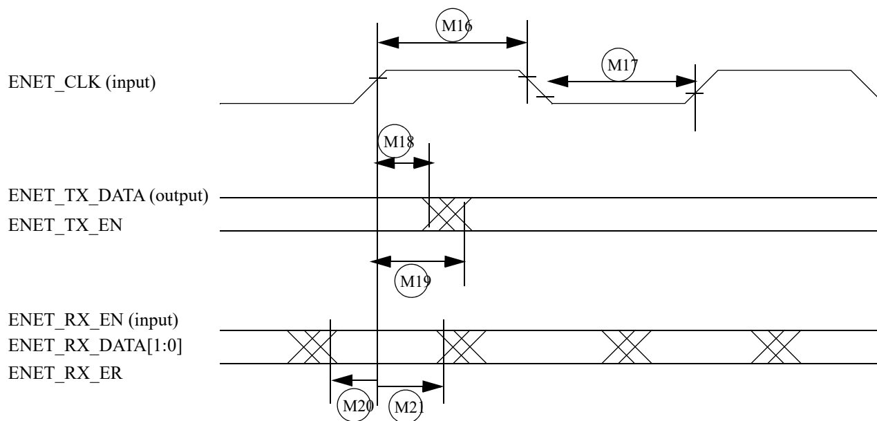
Figure 17. RMI mode signal timing diagram
