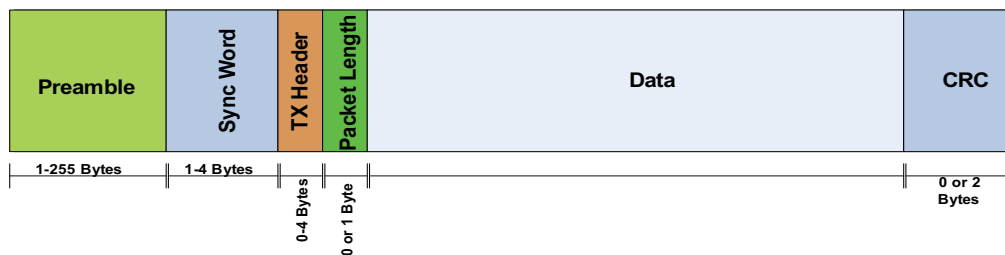
Figure 23.12. Packet Structure
