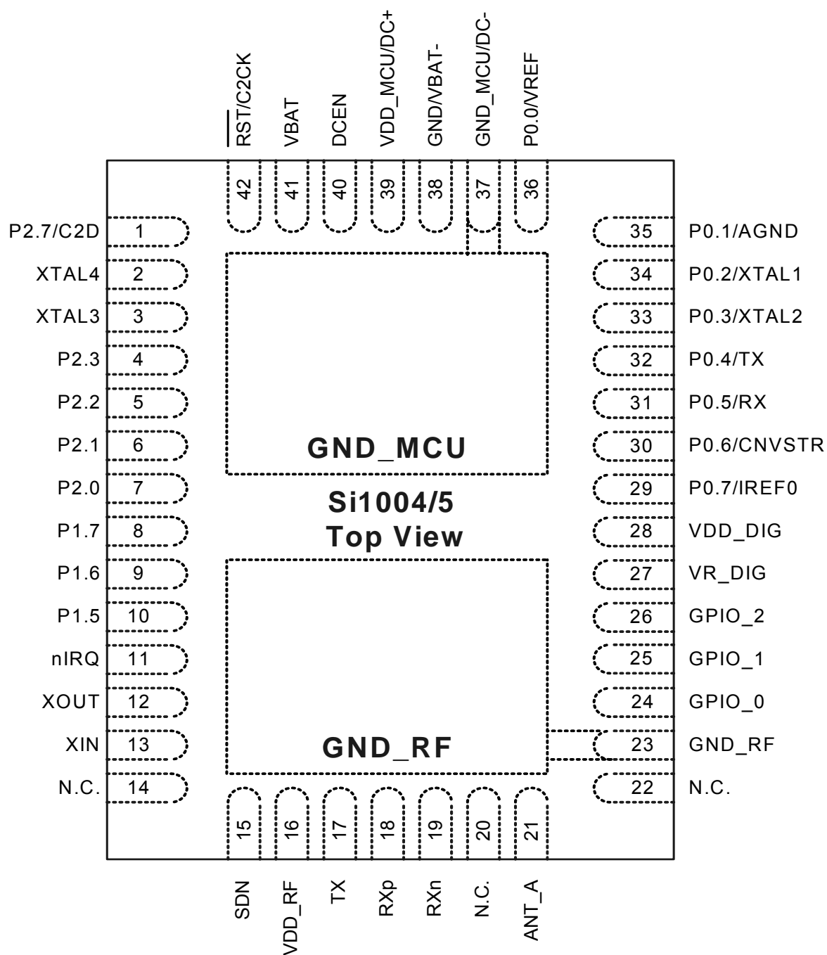
Figure 3.2. Si1004/5-C-GM Pinout Diagram (Top View)
