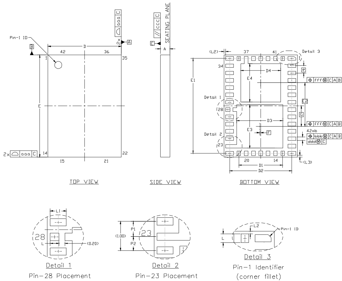
Figure 3.3. QFN-42 Package Drawing (Si1000/1/2/3/4/5-C-GM)
