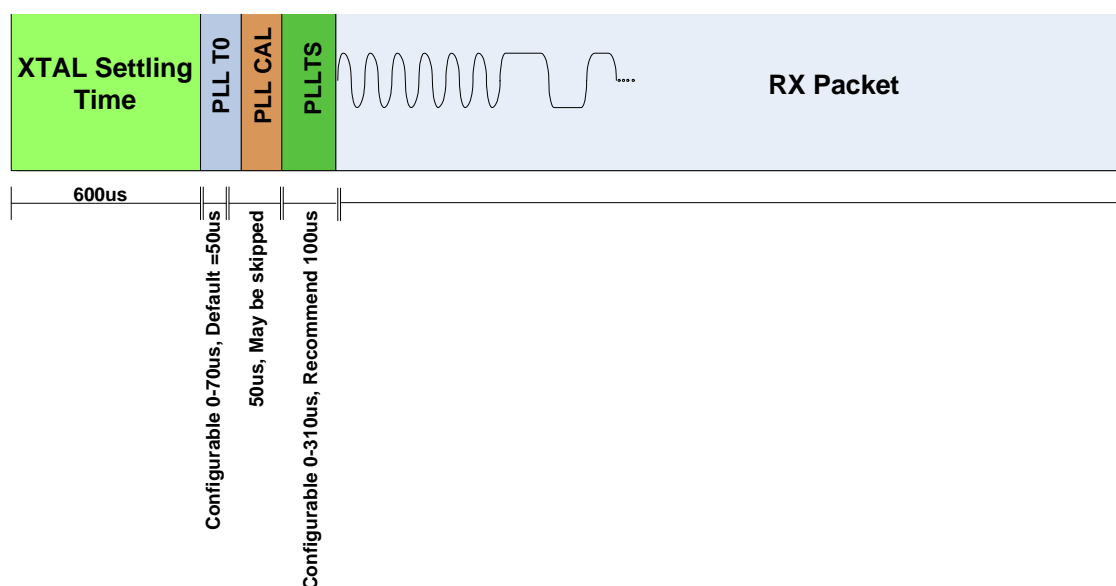
Figure 23.3. RX Timing
