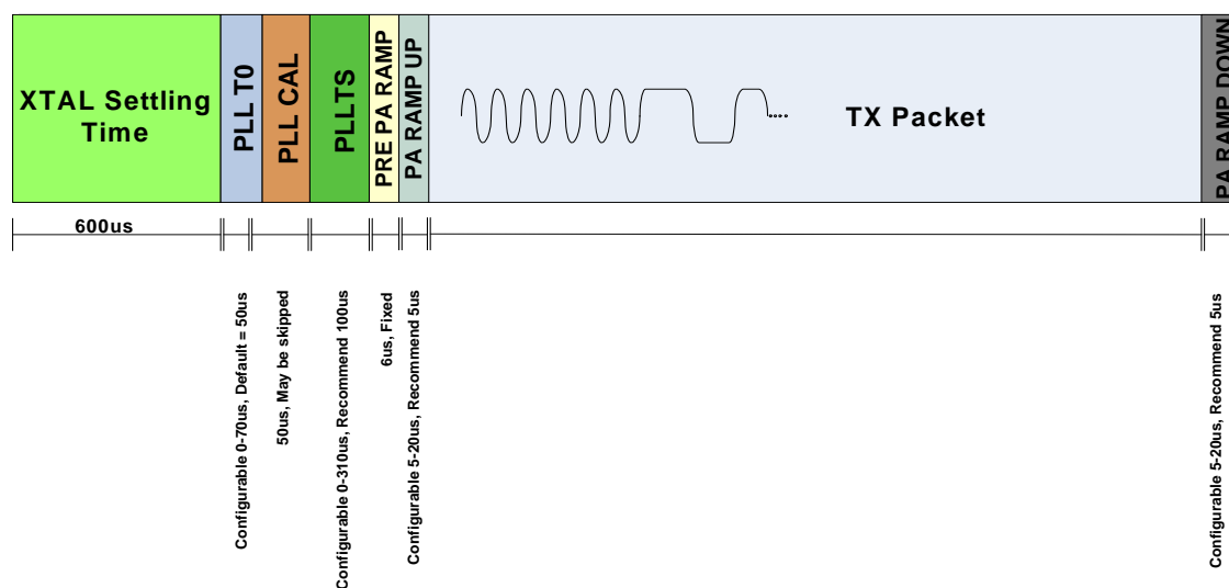
Figure 23.2. TX Timing
