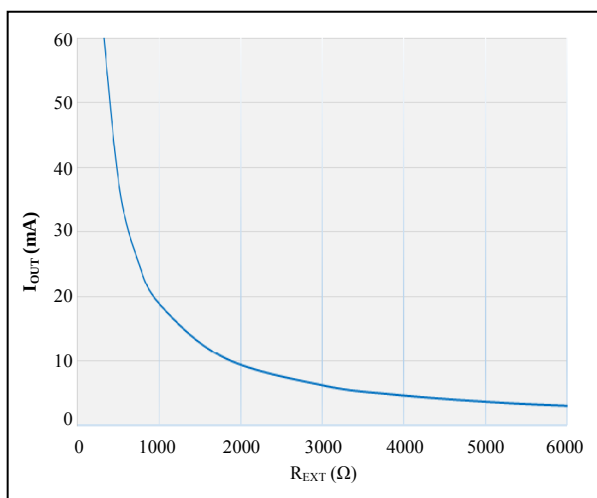
Figure 5 I_{OUT} vs. R_{EXT}
