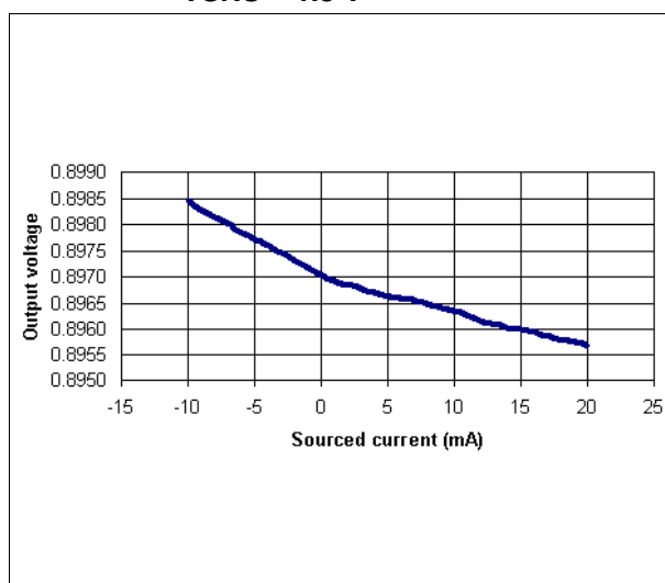
Figure 13. VTTREF load regulation, 0.9 V, V_{SNS} = 1.8\text{ V}
