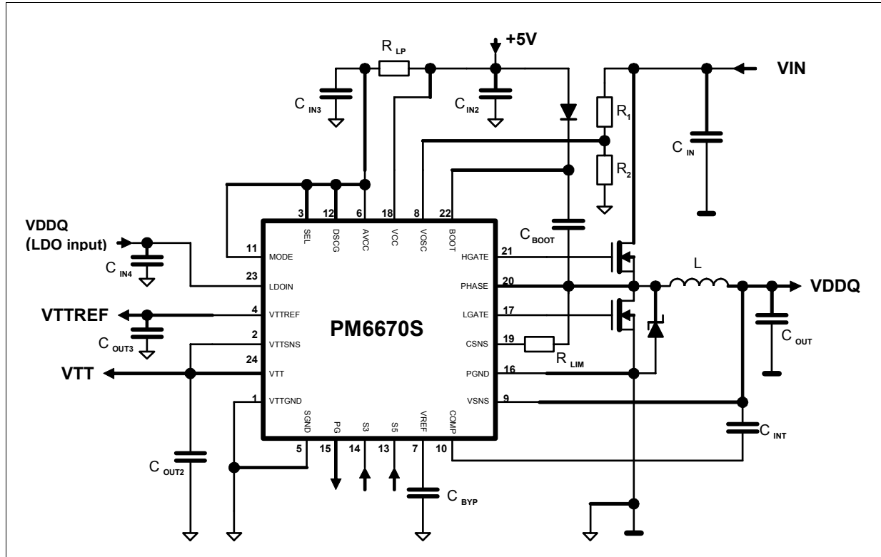
Figure 1. Application circuit
