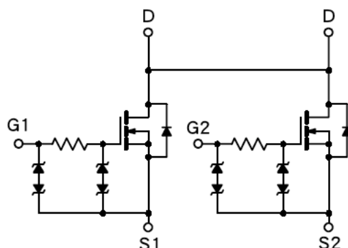
Dual N-Channel MOSFET
