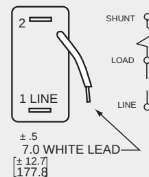
Shunt Trip Single Pole
