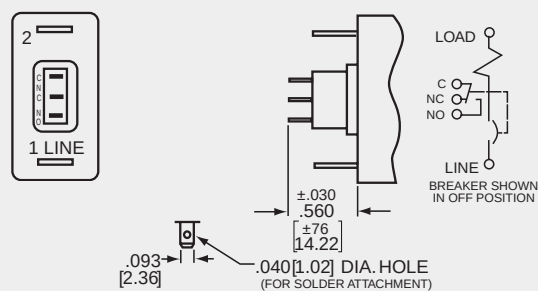
Auxiliary Switch (Note B) Single Pole
