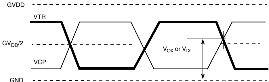
Figure 15. DDR2 and DDR3 SDRAM Differential Timing Specifications
