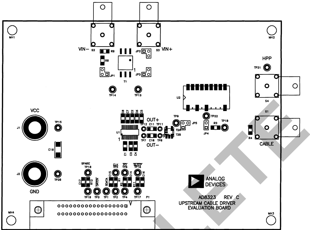
Figure 10. Evaluation Board—Assembly (Component Side)
