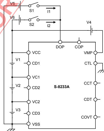
Test circuit 4
