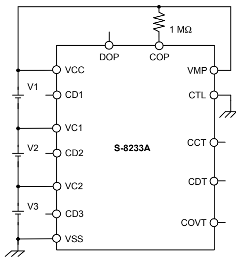
Test circuit 1
