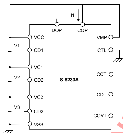
Test circuit 9
