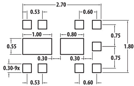
Land Pattern
