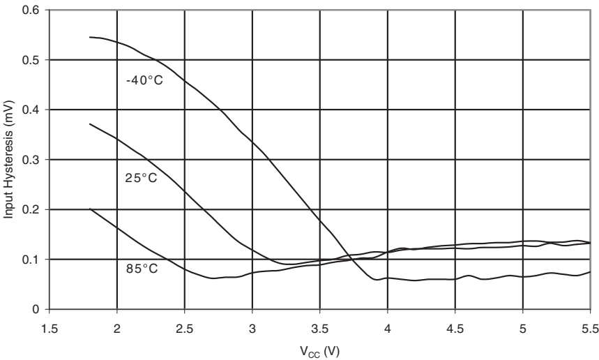
Figure 30-122. Reset Pin Input Hysteresis vs. V_{CC} .
