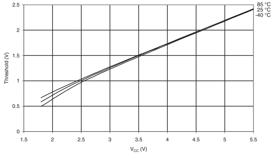
Figure 30-118. I/O Pin Input Threshold Voltage vs. V_{CC} ( V_{IL} , I/O Pin read as '0').
