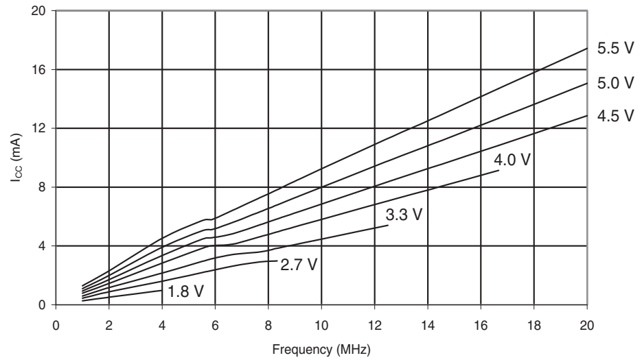
Figure 30-2. Active Supply Current vs. Frequency (1 - 20 MHz).
