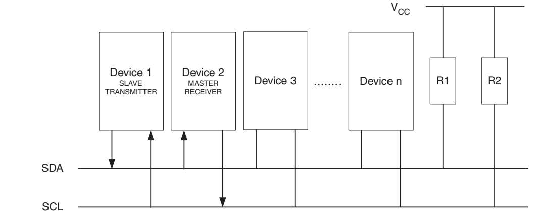
Figure 22-17. Data Transfer in Slave Transmitter Mode
