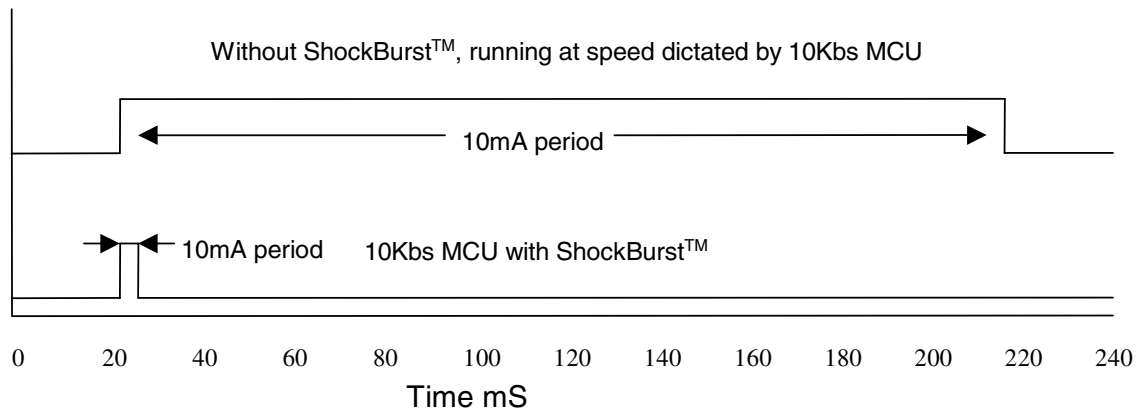
Figure 4-3 RF Current consumption with & without ShockBurst™ technology
