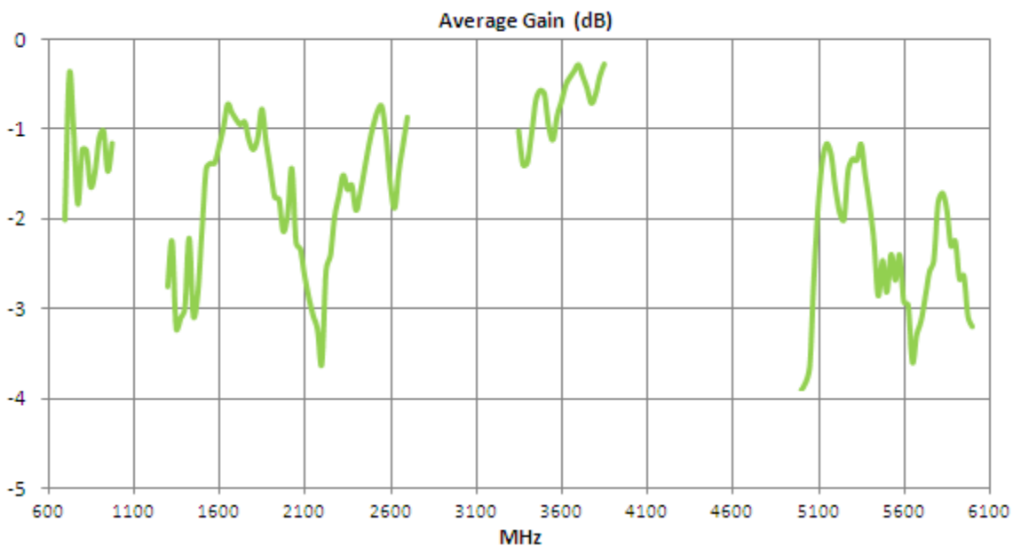
Figure 6. Average Gain of FXUB66 UWB Antenna.
