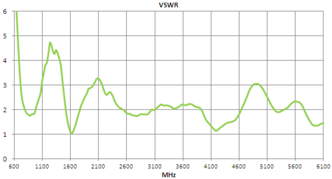
Figure 3. VSWR of FXUB66 UWB Antenna.
