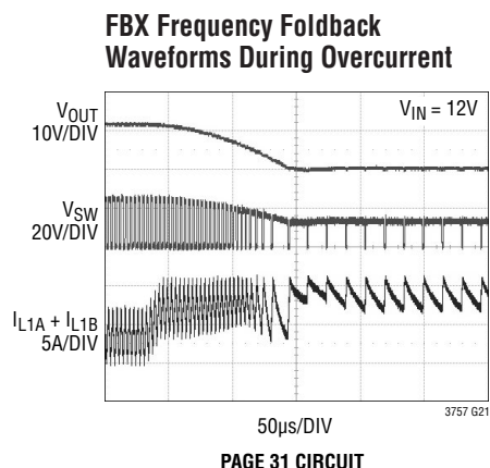
PAGE 31 CIRCUIT
