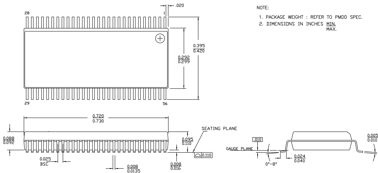
Figure 12. 56-pin SSOP (300 Mils) O563 Package Outline, 51-85062
