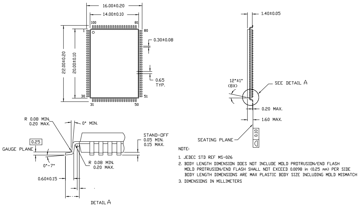
Figure 11. 100-pin TQFP (14 × 20 × 1.4 mm) A100RA Package Outline, 51-85050
