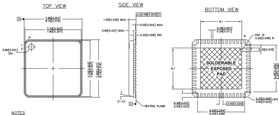
Figure 13. 56-pin QFN 8 × 8 mm LF56A
