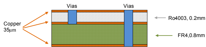
BGAx24N6_application_board_sideview.vsd
