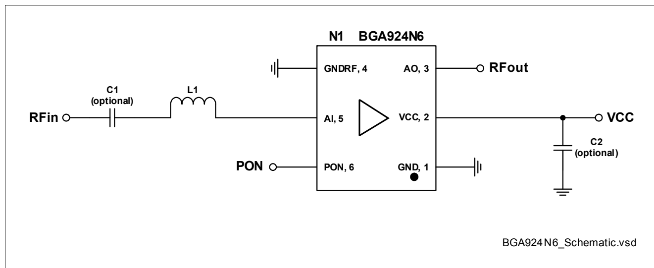
Figure 2 Application Schematic BGA924N6
