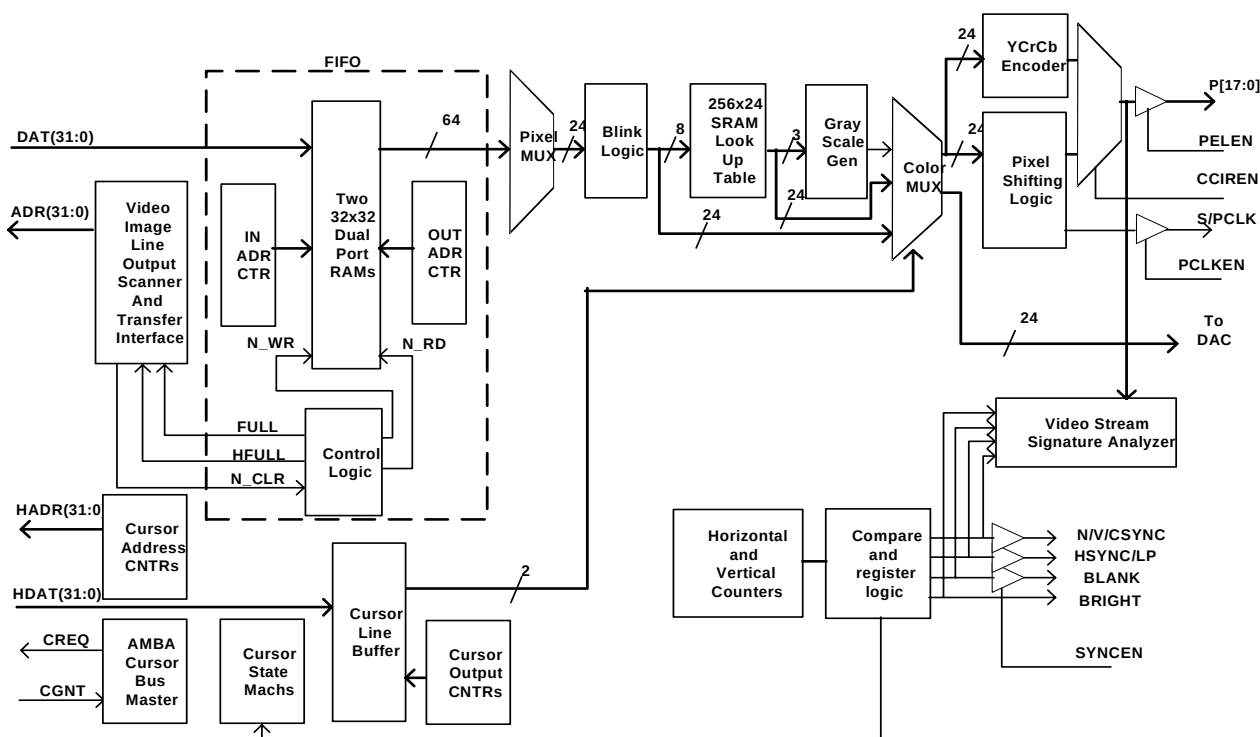
Figure 7-1. Raster Engine Block Diagram
