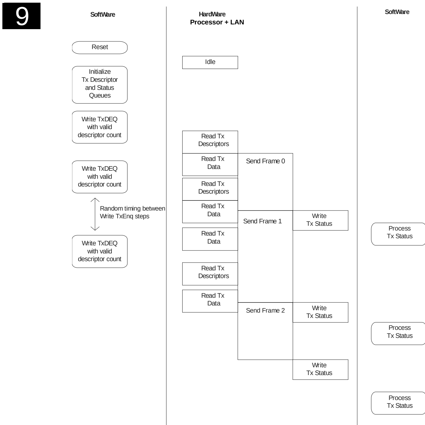
Figure 9-17. Transmit Descriptor Data/Status Flow
