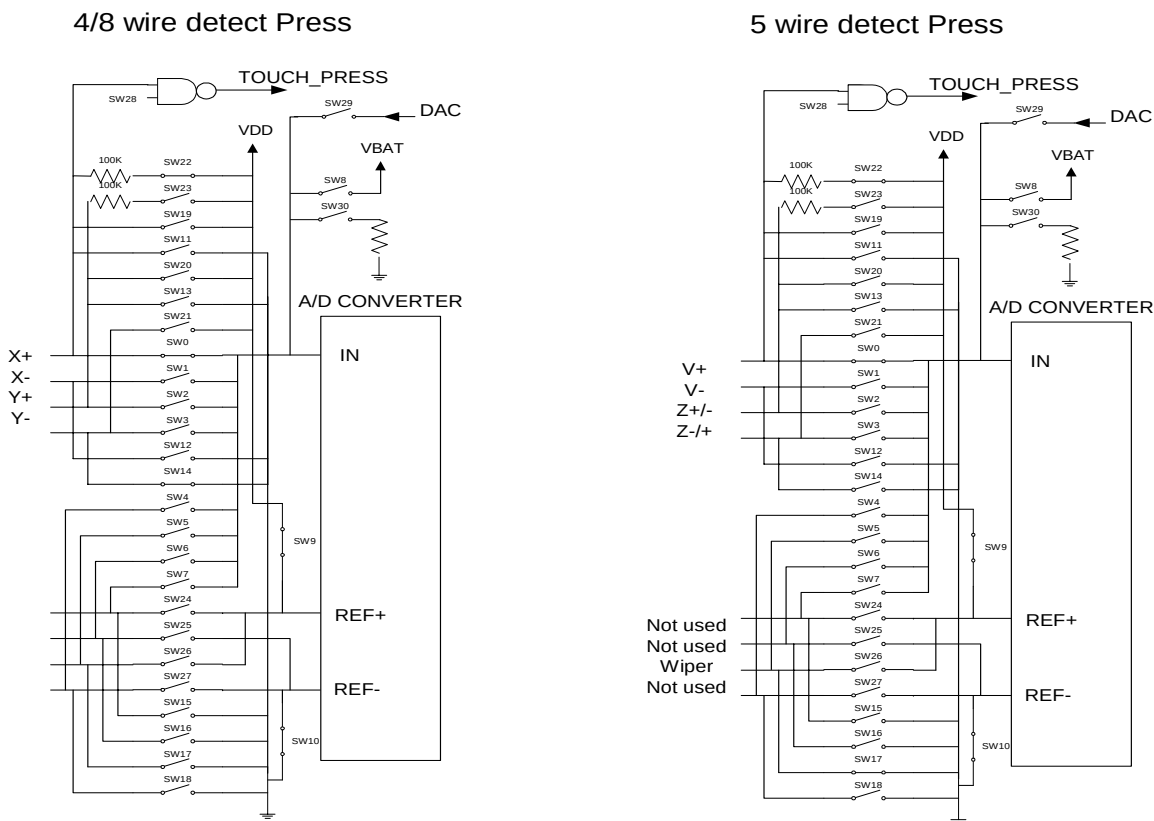
Figure 25-7. Power Down Detect Press Switching Diagram
