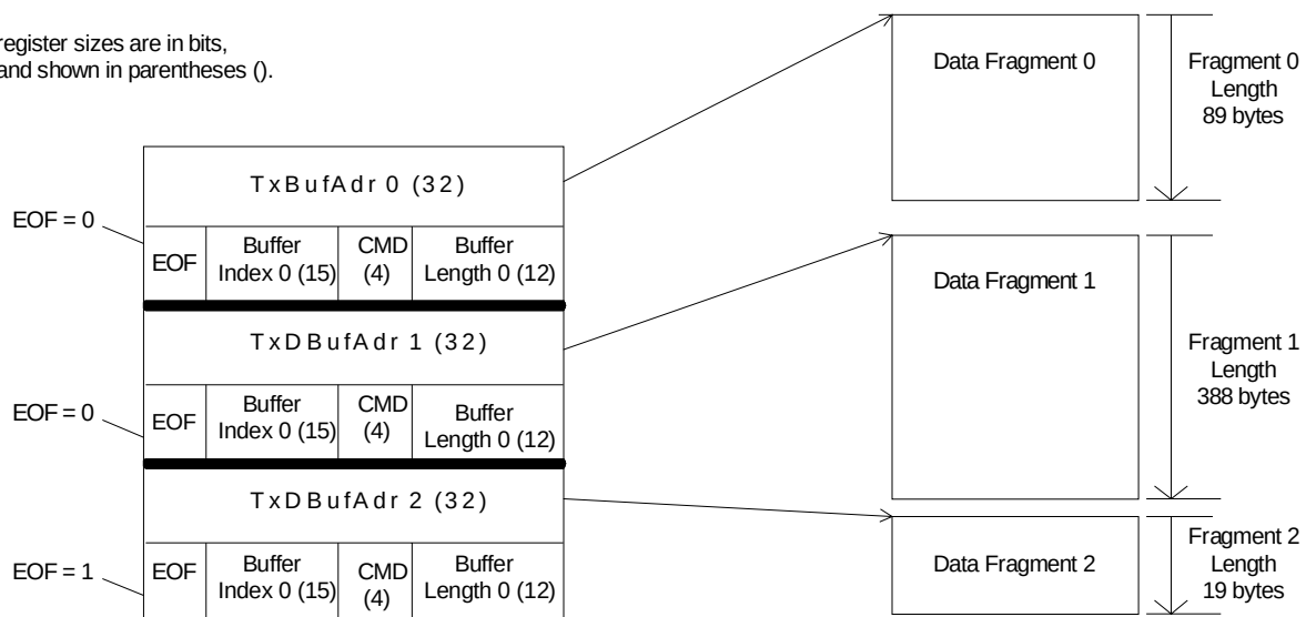
Figure 9-14. Multiple Fragments Per Transmit Frame
