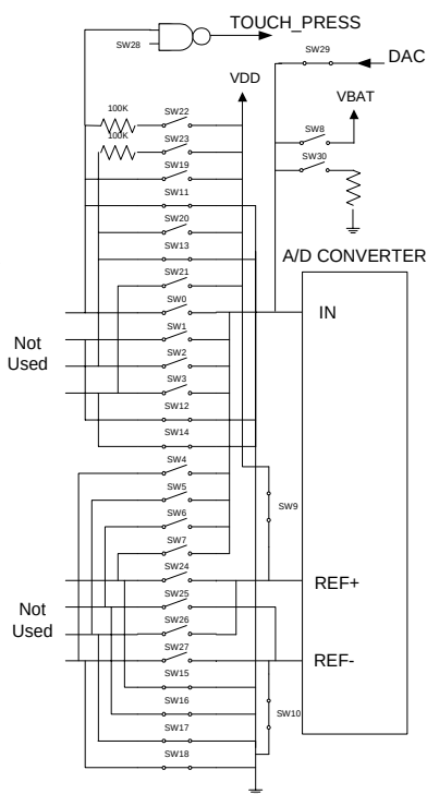
Figure 25-8. Other Switching Diagrams
