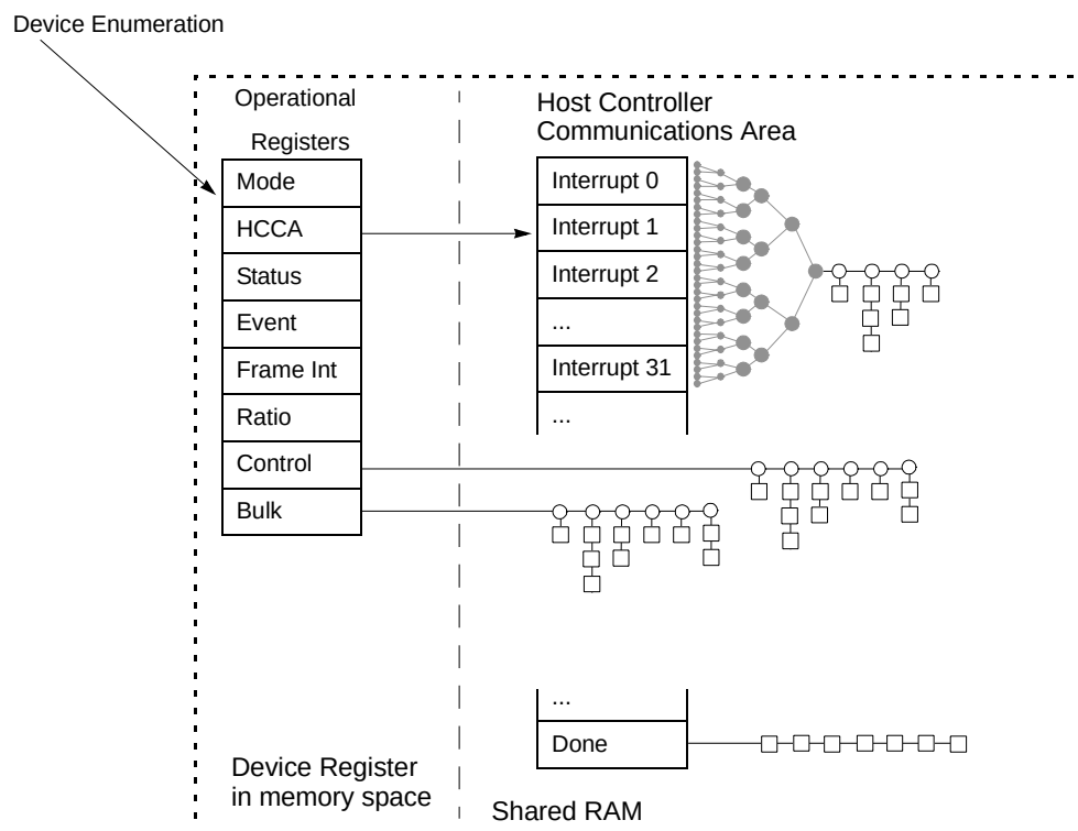
Figure 11-2. Communication Channels
