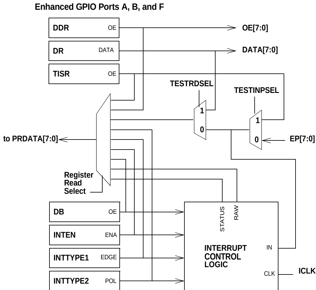
Figure 28-3. Signal Connections Within the Enhanced GPIO Port Control Logic (Ports A, B, F)
