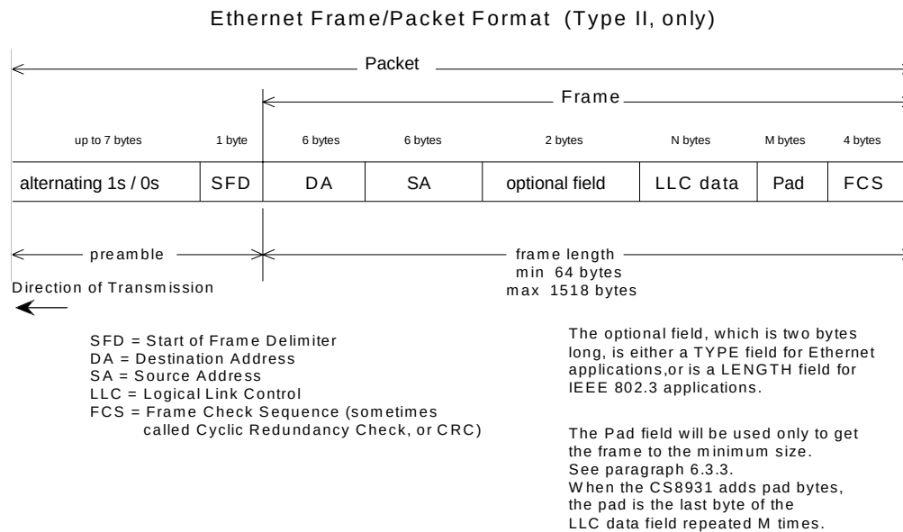
Figure 9-2. Ethernet Frame / Packet Format (Type II only)
