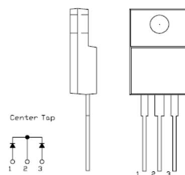
OUTLINE DRAWING
