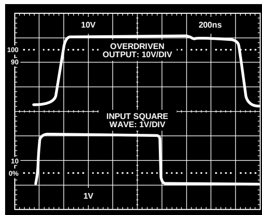
Figure 34. Overdrive Recovery
