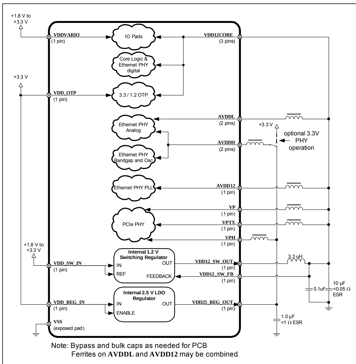
FIGURE 4-1: LAN7430 POWER CONNECTIVITY ON-CHIP REGULATORS ENABLED
