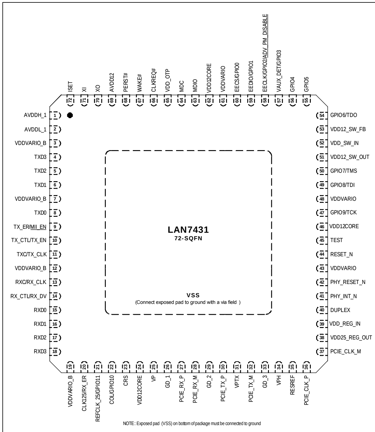
FIGURE 3-2: LAN7431 PIN ASSIGNMENTS
