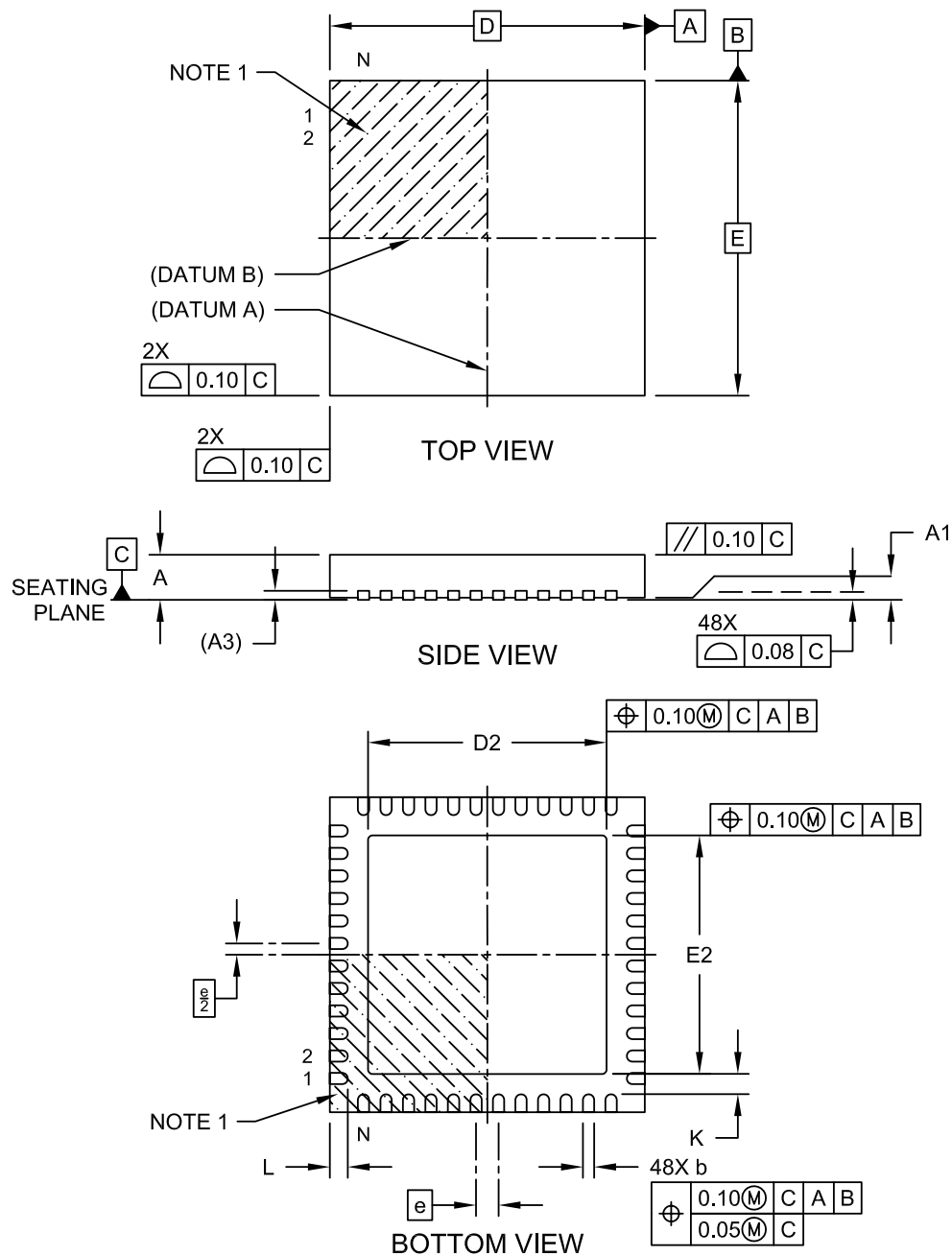
FIGURE 8-1: 48-SQFN PACKAGE (DRAWING)
