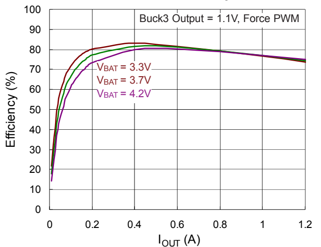
Buck3 Efficiency
