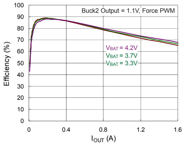
Buck2 Efficiency
