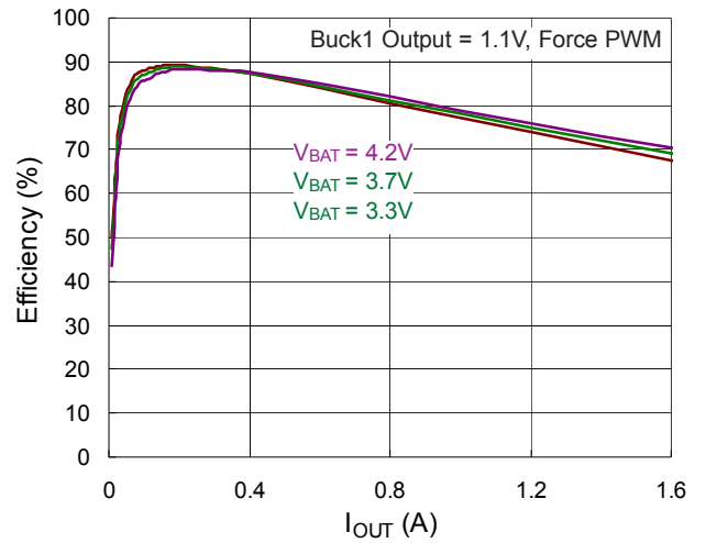
Buck1 Efficiency
