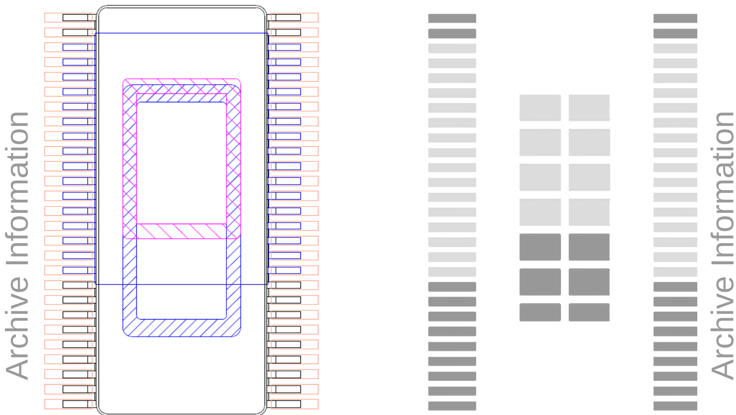
Figure 37. PCB Copper Layer & Solder Stencil Opening Recommendations
