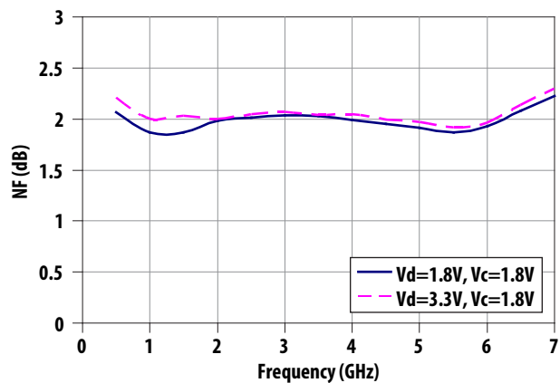
Figure 8. Noise Figure over Vdd [1]
