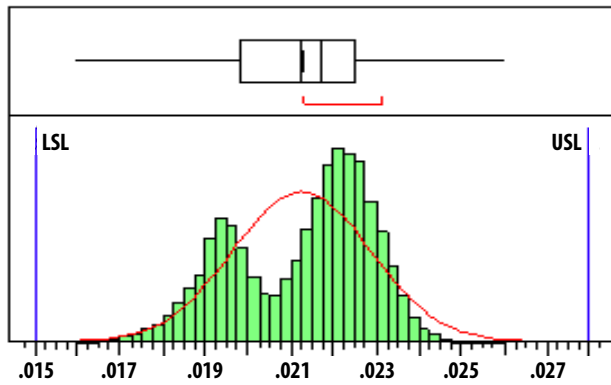
I_d at V_d=V_c=1.8\text{ V} , LSL=15mA, Mean=21mA, USL=28mA
