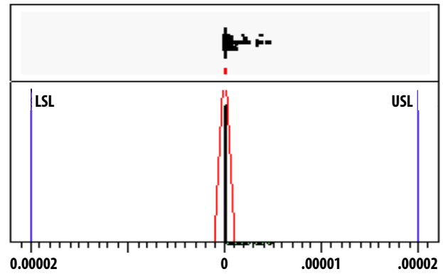
I_{d\_Off} at V_d=1.8\text{ V} & V_c=0\text{ V} , Mean=0.025uA, USL=20uA
