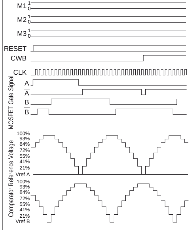
2W1-2 Phase Excitation Timing Chart (M3=1)
