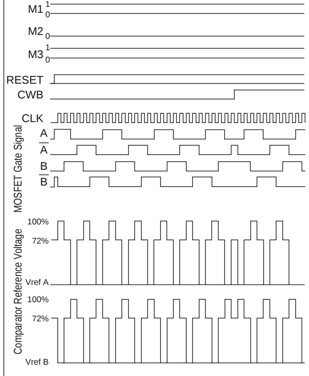
1-2 Phase Excitation Timing Chart (M3=1)
