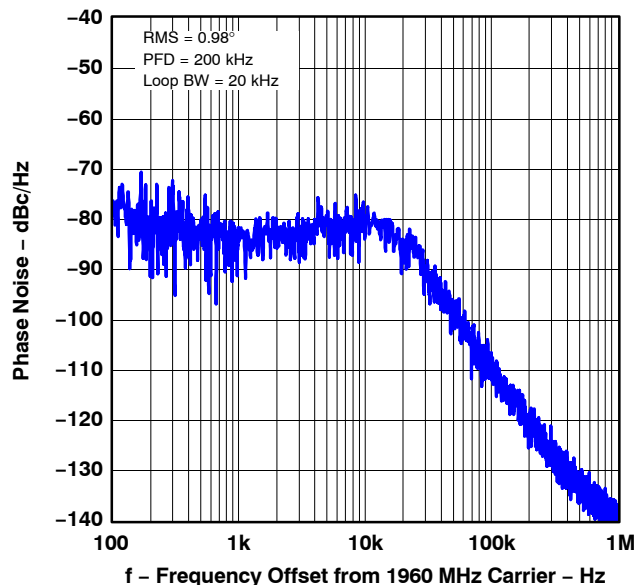
Figure 17. Integrated Phase Noise (RFOUT = 1960 MHz)
