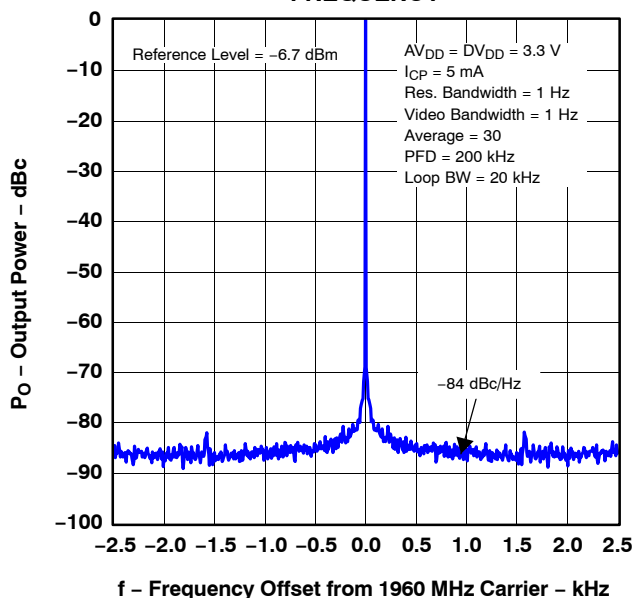
Figure 16. Phase Noise (RFOUT = 1960 MHz)
