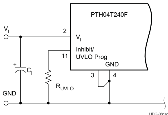
Figure 16. Undervoltage Lockout Adjustment Resistor Placement
