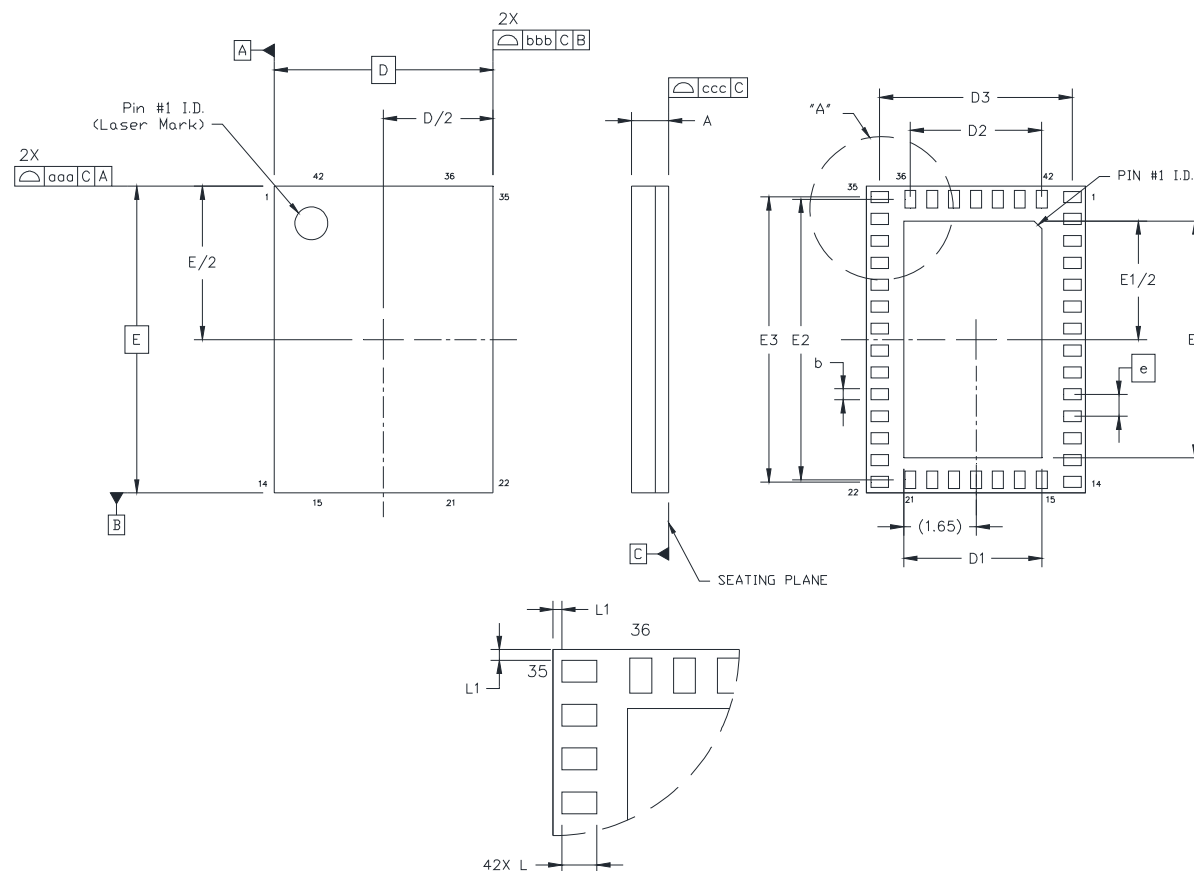
Figure 3.3. LGA-42 Package Drawing (Si1000/1/2/3/4/5-E-GM2)
