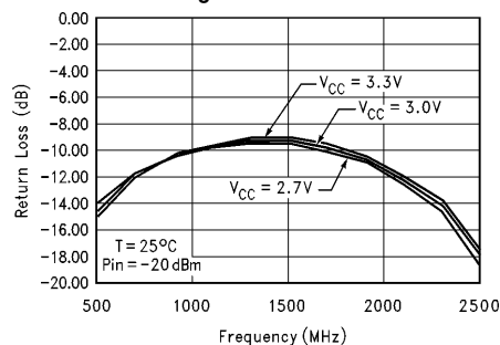
LNA Output Return Loss vs Frequency with Voltage as a Parameter
