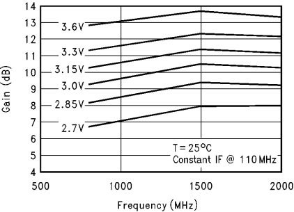
Mixer Gain (Double Sideband) vs Frequency with Supply Voltage as a Parameter
