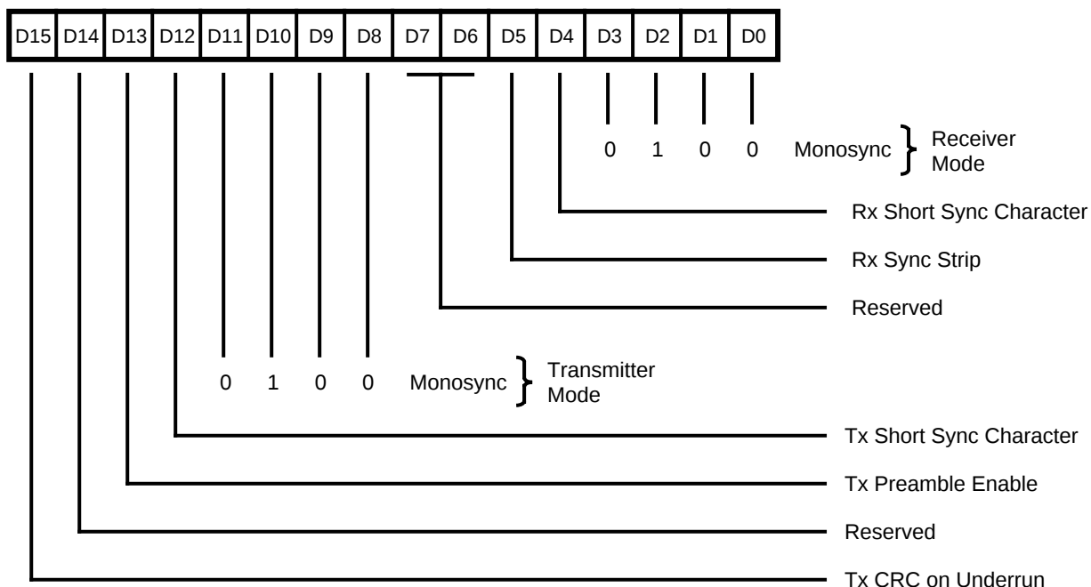
Figure 41. Channel Mode Register, Monosync Mode
