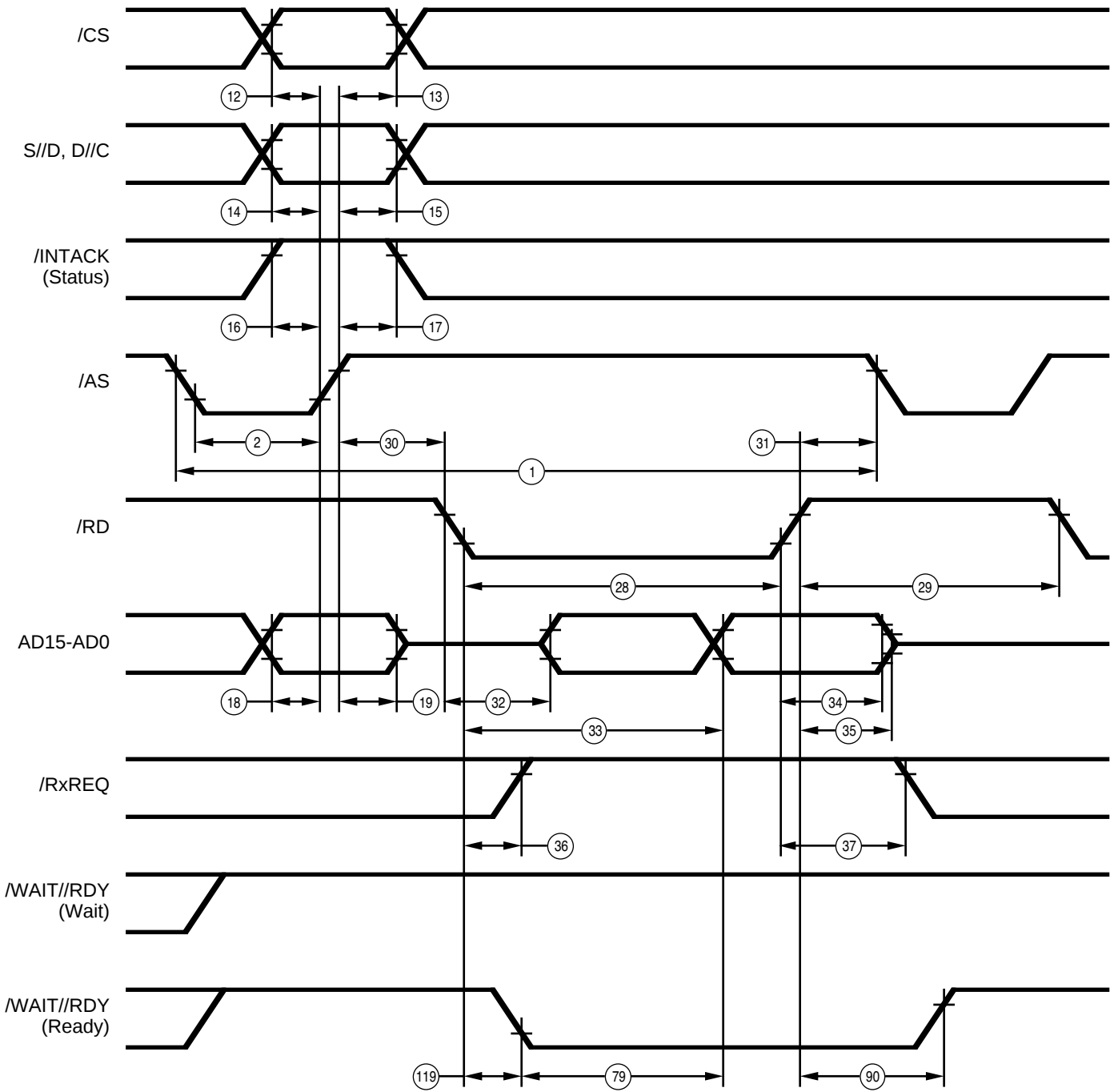
Figure 87. Multiplexed \overline{\text{RD}} Read Cycle
