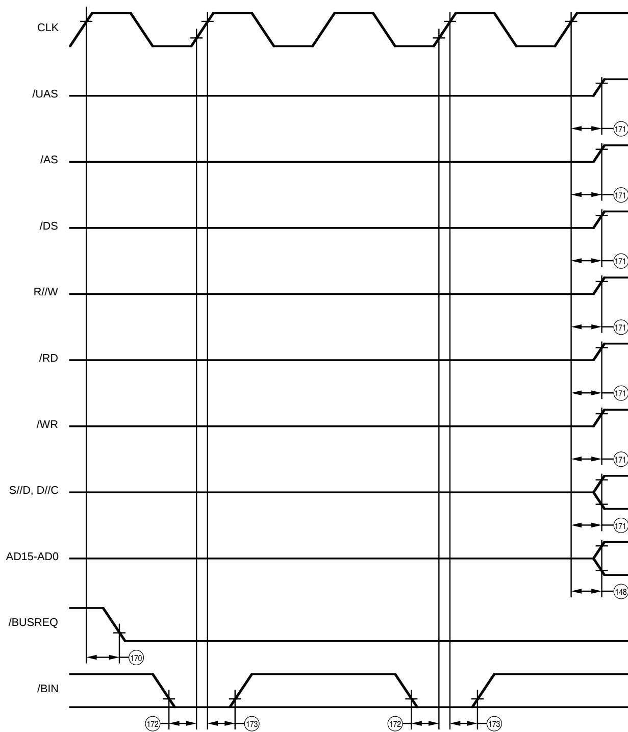
Figure 101. DMA Start-Up
