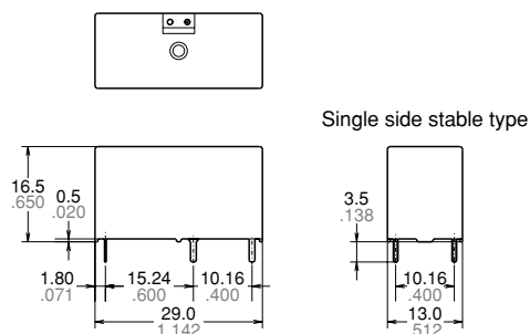
External dimensions
