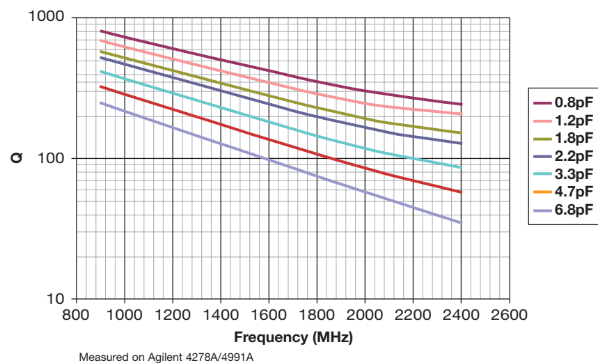
Accu-P® 0603 Typical Q vs Frequency
