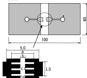
Fig.1 (in : mm)
