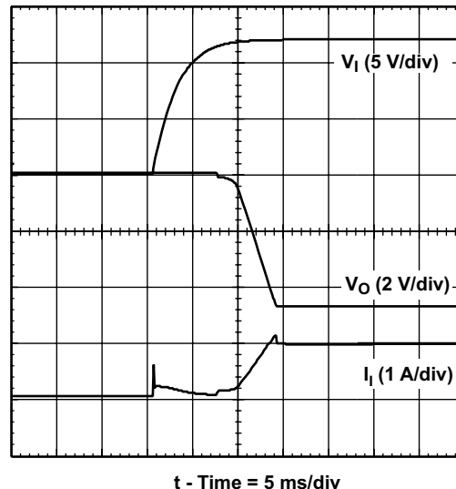
Figure 18. Power-Up Waveforms
