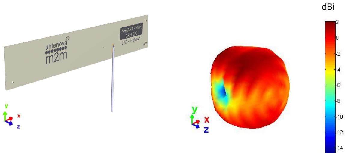
3D pattern at 745 MHz
