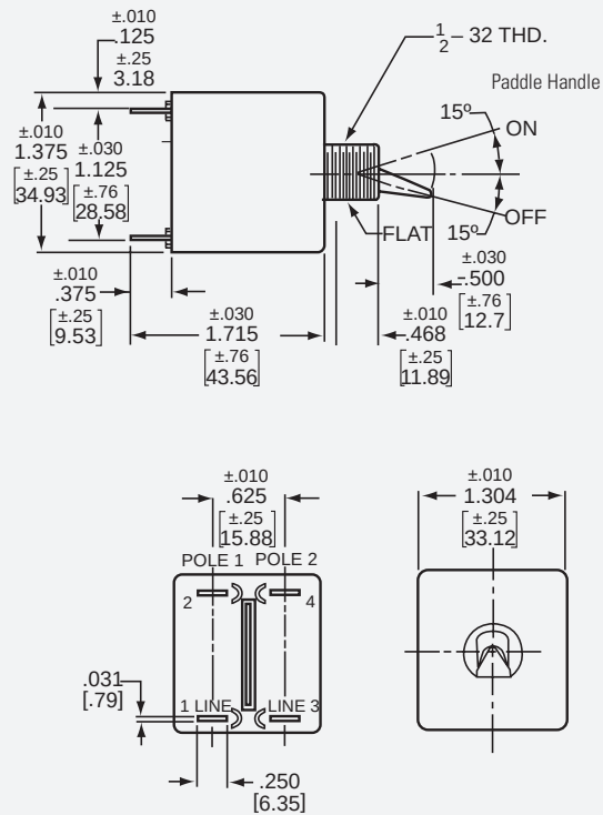
Two Pole, Toggle
