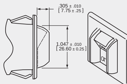
Handle Guards, Two Pole
