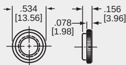
3/8 - 32 Panel Nut Bright Nickel
