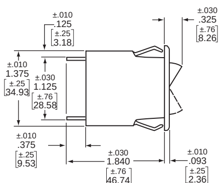
Rocker, Single Pole
