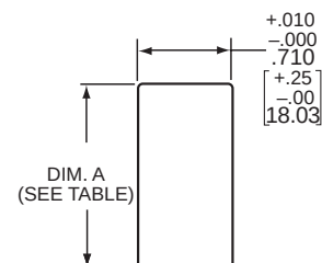
Mounting Detail
