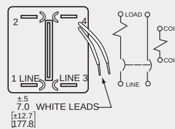
Two Pole (1 pole relay)
