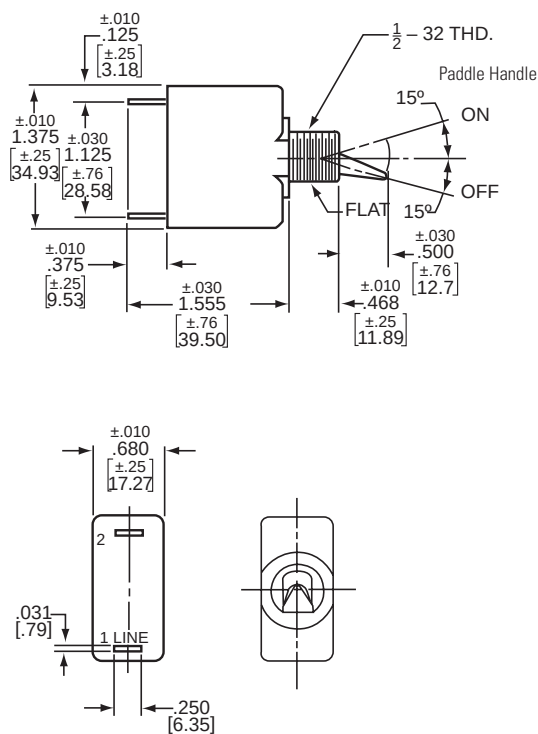
Single Pole, Toggle
