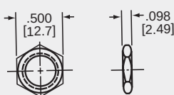
3/8 - 32 Hex Nut Bright Nickel
