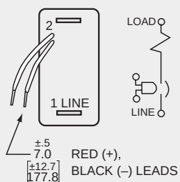
Illuminated Handle Single Pole
