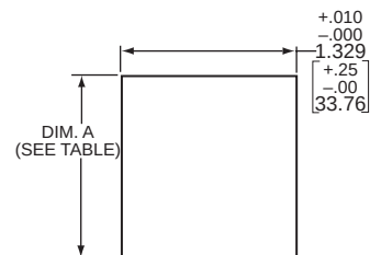
Mounting Detail
