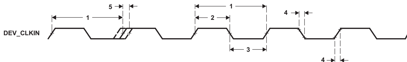
Figure 7-6. DEV_CLKIN Timing
