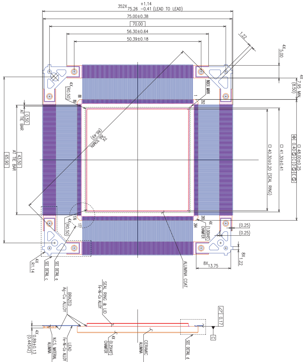
Figure 11 • RTG4 CQ352—Cavity Up without Heat Sink: Top View
