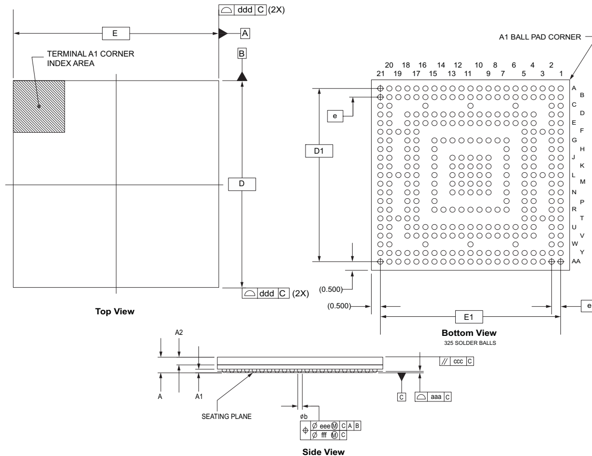
Figure 65 • Package Outline of FCS325 (Option 1)
