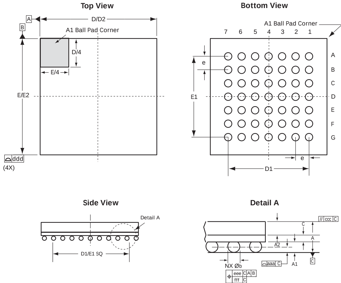
Figure 57 • Package Outline of CS49
