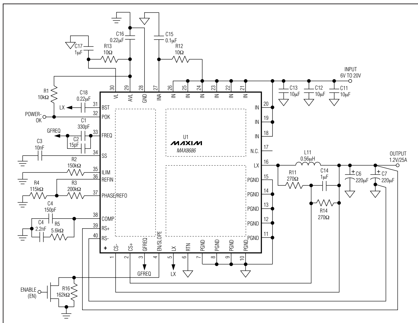
Figure 2. Single-Phase Application Circuit Operating at V_{IN} = 12\text{V}
