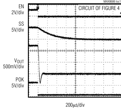
SHUTDOWN WITH EN CONTROL ( I_{OUT} = 10A )
