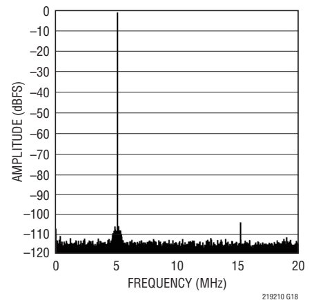
LTC2191: 64k Point FFT, f_{IN} = 5\text{MHz} , -1dBFS, 40Mps
