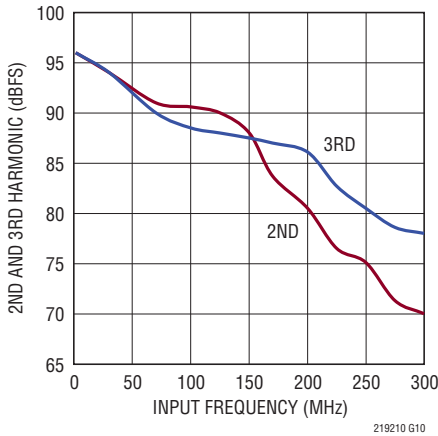
LTC2192: 2nd, 3rd Harmonic vs Input Frequency, -1dBFS, 65Mps, 2V Range
