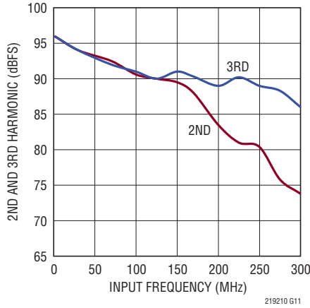
LTC2192: 2nd, 3rd Harmonic vs Input Frequency, -1dBFS, 65Mps, 1V Range
